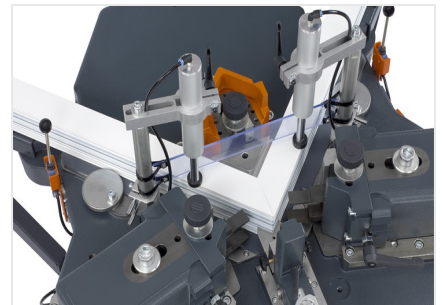
Hoekverbindingpers EP 124
