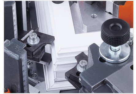
Hoekverbindingpers EP 124
