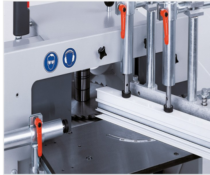
端面铣床AF 222/02
