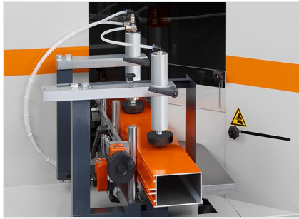
Notching saw AKS V-550
