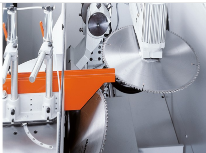
Notching saw AKS 134/00
