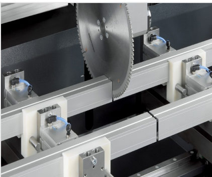
Profile machining centre SBZ 131 eluCam
