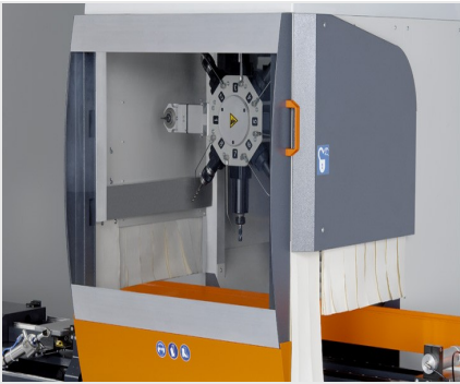
a-Profile machining centre SBZ 131 eluCam
