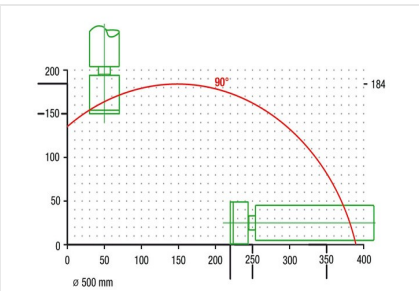
Automatic saw SAS 142/44
