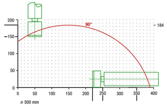
Automatic saw SAS 142/44
