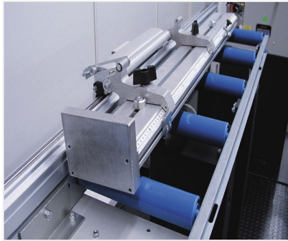
Stop and measurement system MMS 200
