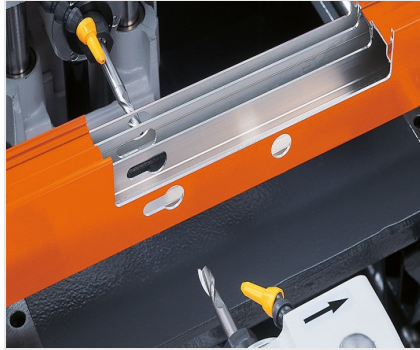
3-spindle copy router KF 178/10
