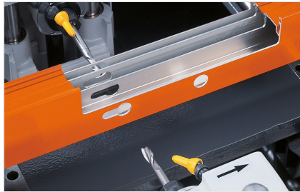
3-spindle copy router KF 178/10
